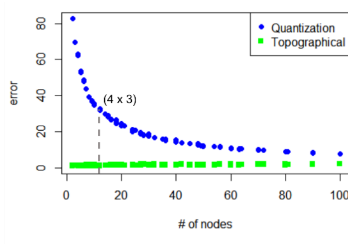
Figure 13: Quantization and topographical errors for SOM at various grid sizes.
