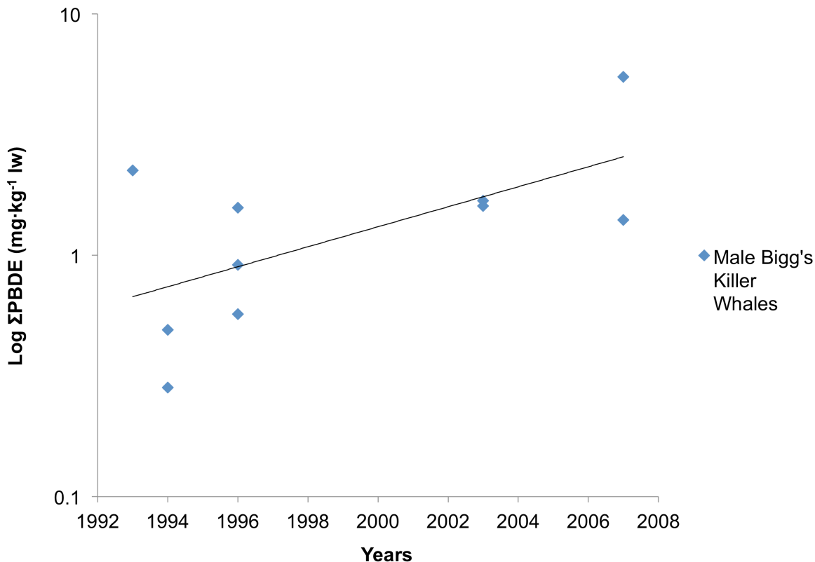
Figure 4.21 Log concentrations of total polybrominated diphenyl ethers (ΣPBDEs) in male Bigg's killer whales in units of mg·kg -1 lipid weight (lw; ◆) versus time in years. The solid line represents the linear regression of the log transformed concentrations of ΣPBDEs in killer whales and time.
