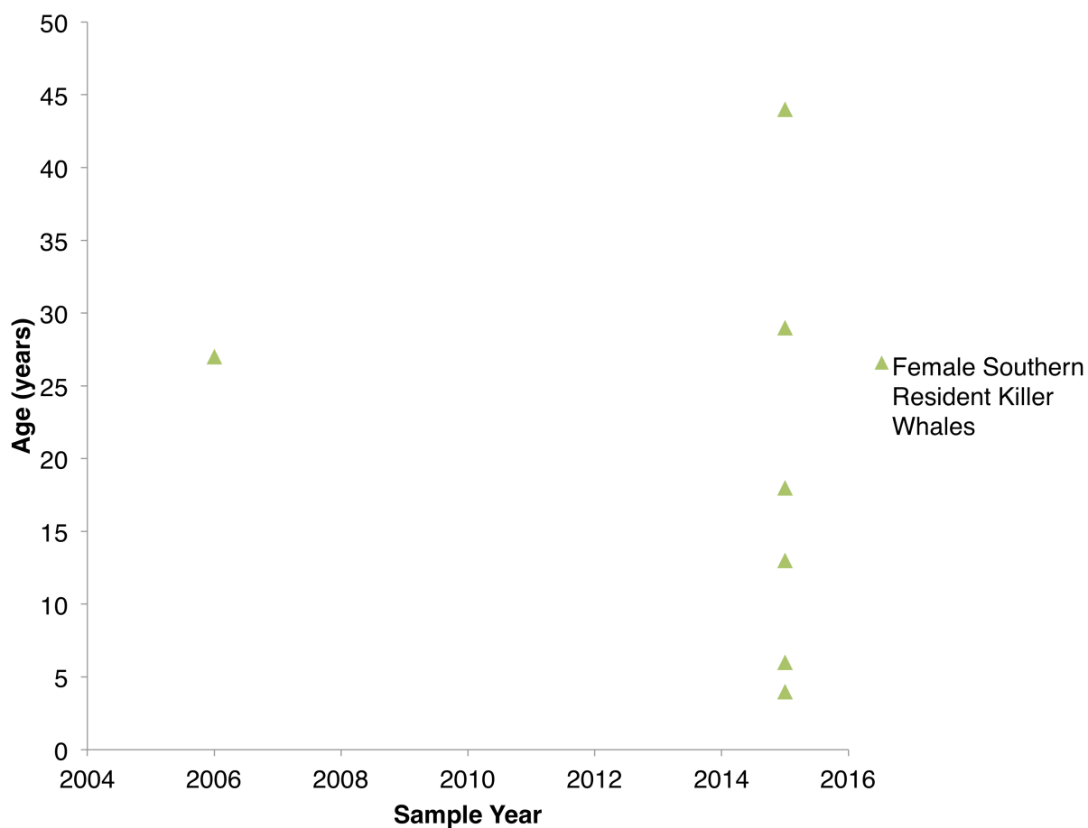
Figure 4.26 The age of female southern resident killer whales sampled for total polybrominated diphenyl ethers (ΣPBDEs) plotted against the year in which each killer whale was sampled.
