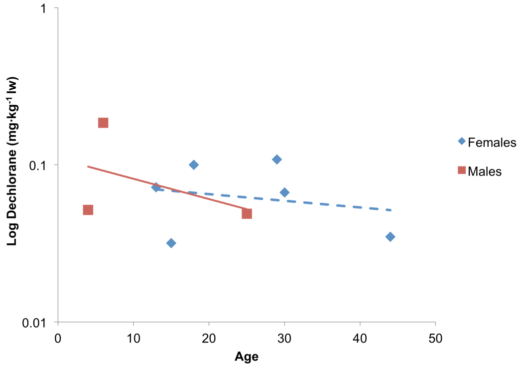
Figure 4.37 The log-transformed concentrations of Dechlorane ( \text{mg}\cdot\text{kg}^{-1} lw) in southern resident killer whales as a function of the ages (in years) of killer whales sampled in 2015. Two linear regression analyses are shown, one for females (◆) and the other for males (■).
