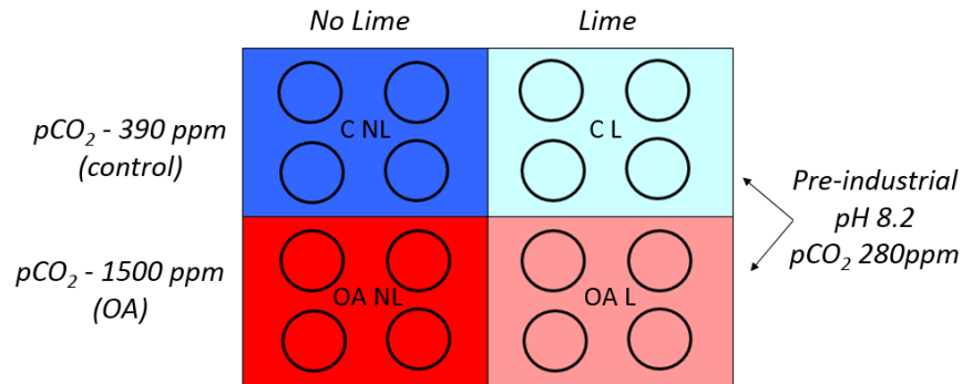
Figure 2: Using a complete randomized design, 16 aquaria (represented by circles) were randomly assigned to four carbonate chemistry treatments (C NL, OA NL, C L, and OA L) for a total of four replicates per treatment
