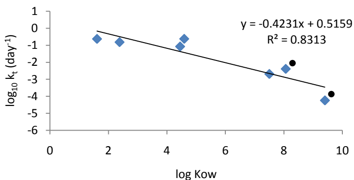
Figure 16. Observed log biodegradation rate ( k_t ) versus \log K_{ow} . • Denotes k_t values which are not statistically significantly different from 0 (DnOP and DiNP).
