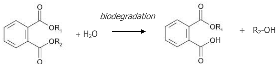
Figure 3. Generalized primary biodegradation reaction for phthalate diesters and primary metabolites (monoester and associated alcohol). Variation of side chain (R 1 , R 2 ) length and branching pattern differentiate between congeners.
